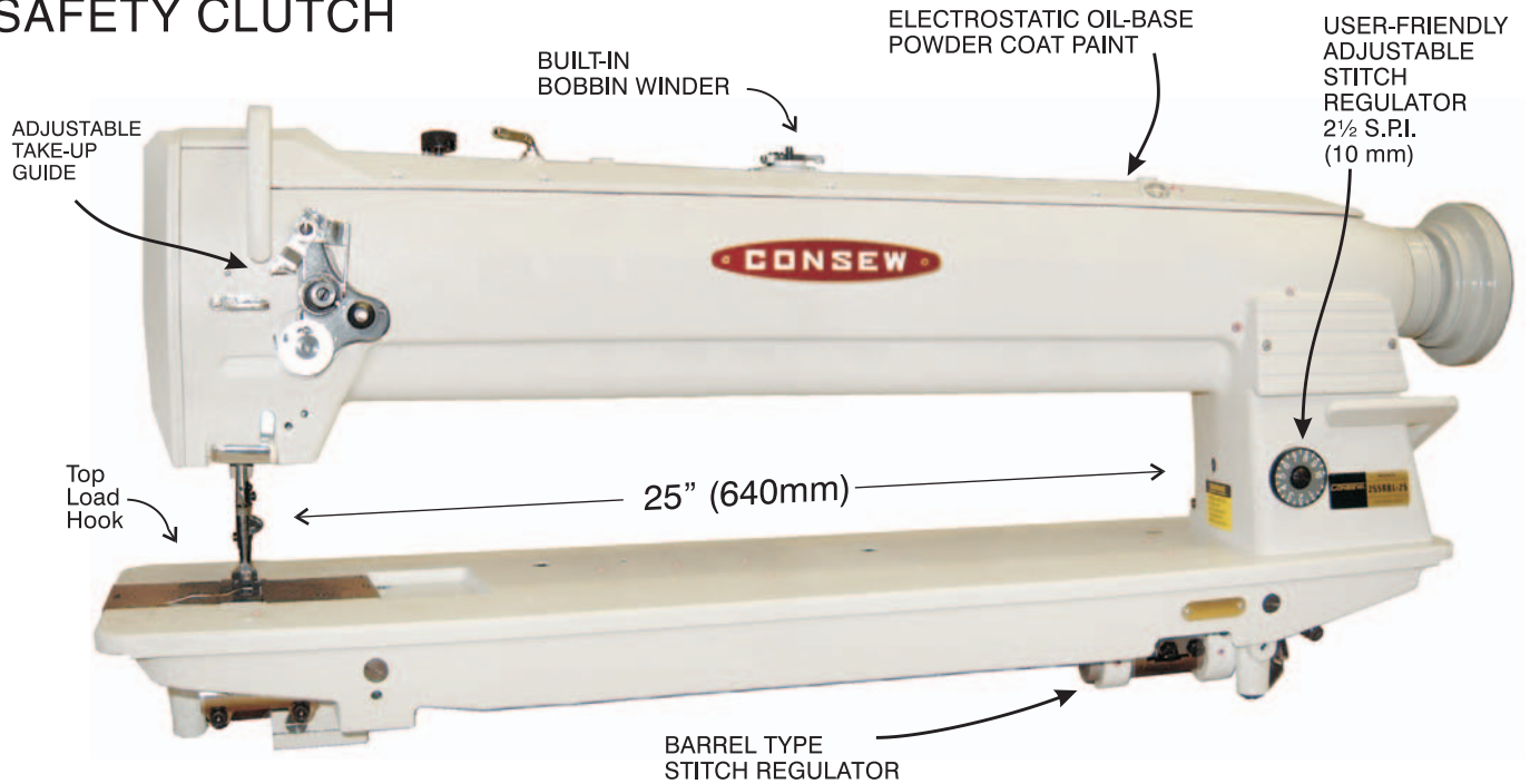
Model 255RBL-25 HEAVY DUTY SINGLE NEEDLE TRIPLE FEED: DROP FEED, NEEDLE FEED AND ALTERNATING (WALKING) PRESSER FEET LOCKSTITCH MACHINE
